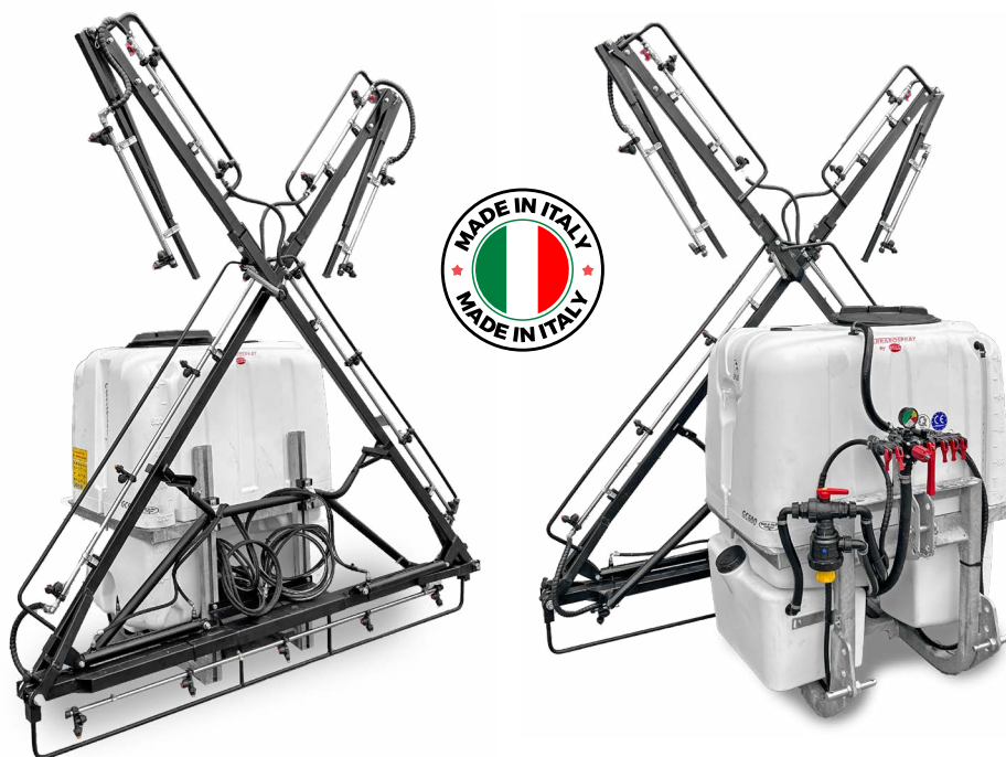
FIELD HYDRO GC-BDI 400-600-1000 L
